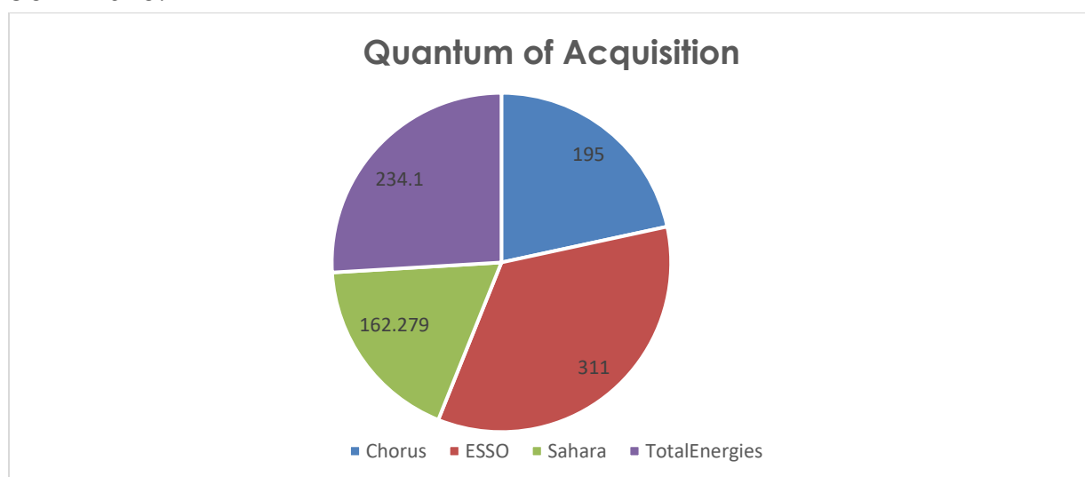
Fig. 3.0: Quantum Acquisition
